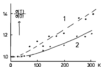
Fig. 5. Temperature dependence of the relative emission band width of the luminescences of solid [Ce^{3+} \subset 2.2.1] (circles) and of solid [Ce^{3+} \subset 2.2.2] (crosses). The drawn and the broken curves represent fit curves, as discussed in the text. \sigma(T) indicates the band width of the individual components of the emission band at the temperature T .
